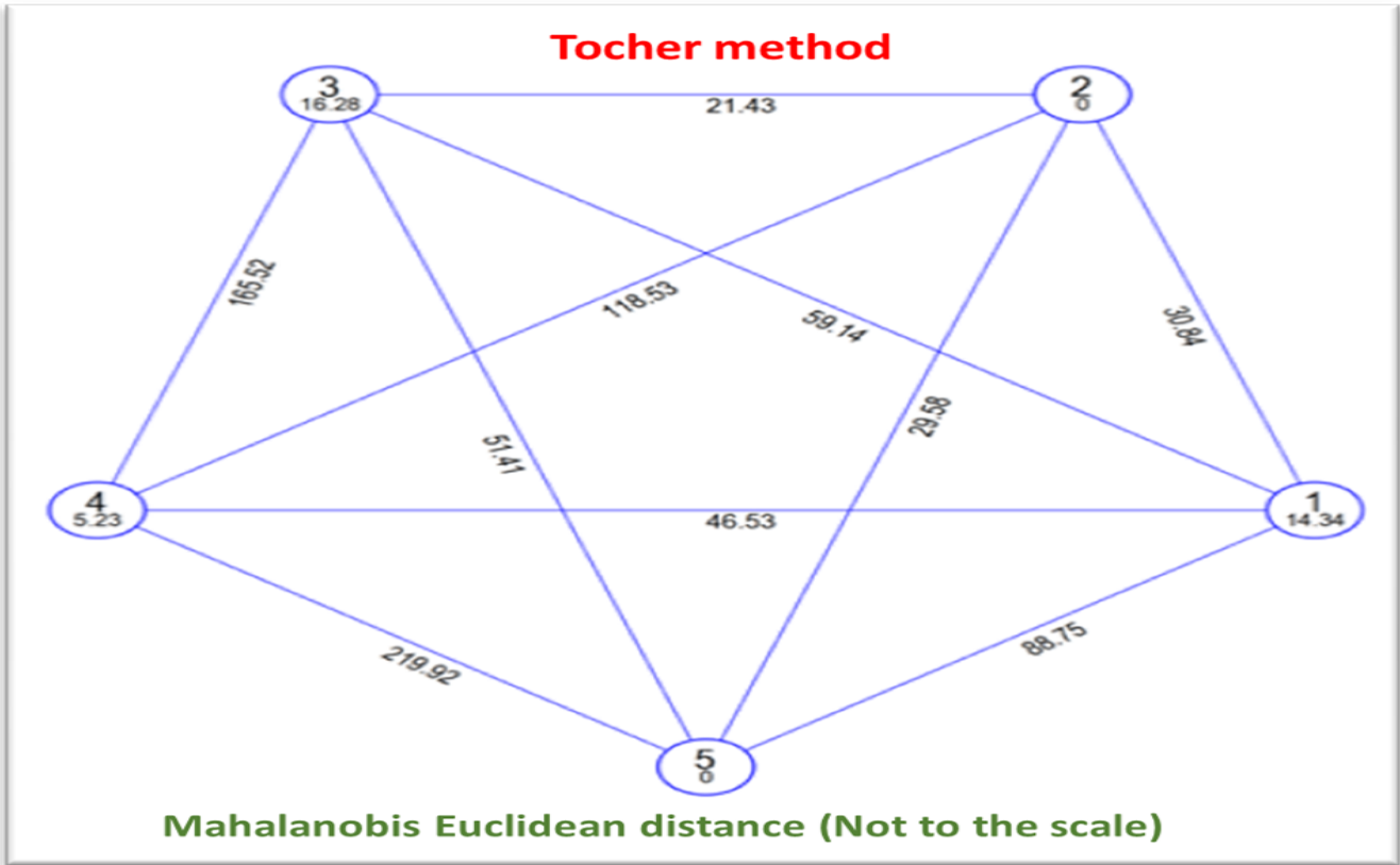
Fig. 6. Intra and inter-cluster distance of thirty maize inbred lines based on Mahalanobis Euclidean distance.
