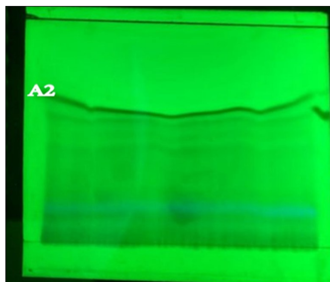
Fig. 4. Preparative layer chromatography was used on the ethyl acetate fraction using a solvent mixture of 55:30:10:5, toluene: ethyl acetate: Formic acid: methanol, under UV light 254 nm, A2 is Pinoresinol.
