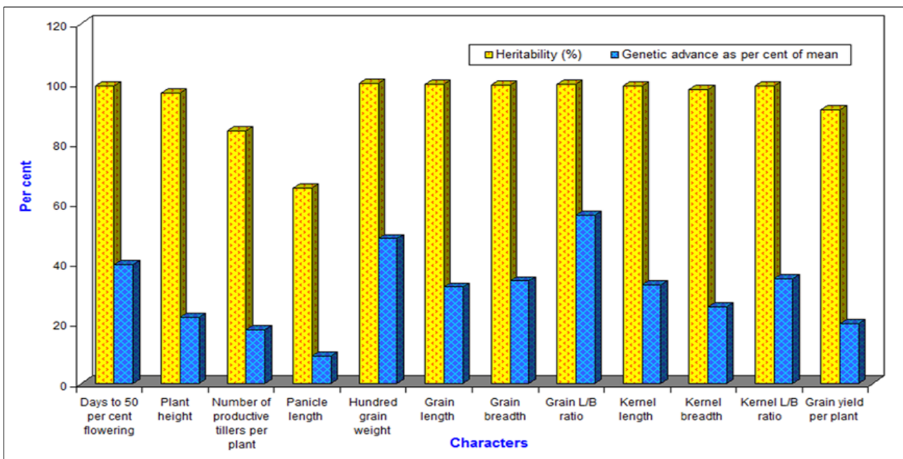
Fig. 3b. Estimated heritability and genetic advance as per cent of mean for various characters in rice.
