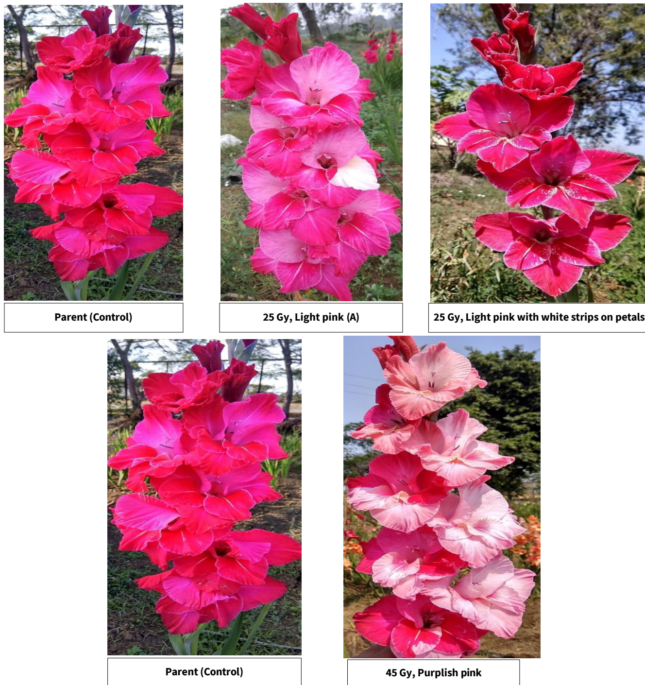
Fig. 3. Effect of gamma irradiation on gladiolus cv. Candyman.
