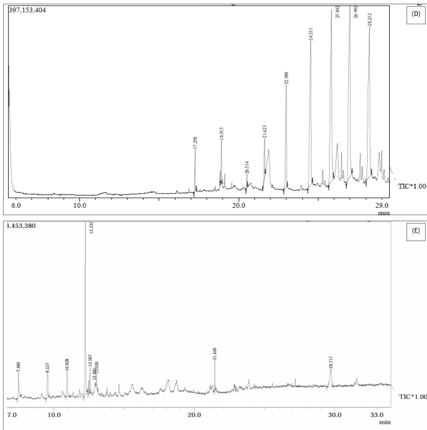
Fig. 2. Gas chromatography-mass spectrometry chromatograms of methanolic extracts of Clitoria ternatea (white-flowered variety). (A) Leaves extract showing dominance of long-chain hydrocarbons and fatty acids such as hexadecanoic acid and pristane; (B) Stem extract characterised mainly by saturated and unsaturated fatty acids; (C) Root extract enriched with aliphatic hydrocarbons; (D) Seed extract containing fatty acids and alkanes; (E) Flower extract dominated by oxygenated compounds including 3-furanmethanol, glycerol and heterocyclic compounds.
