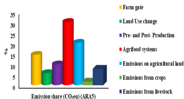
Fig. 1. Emission share of CO 2 equivalent of different categories [Data sourced from FAOSTAT for the year 2021] (9)
