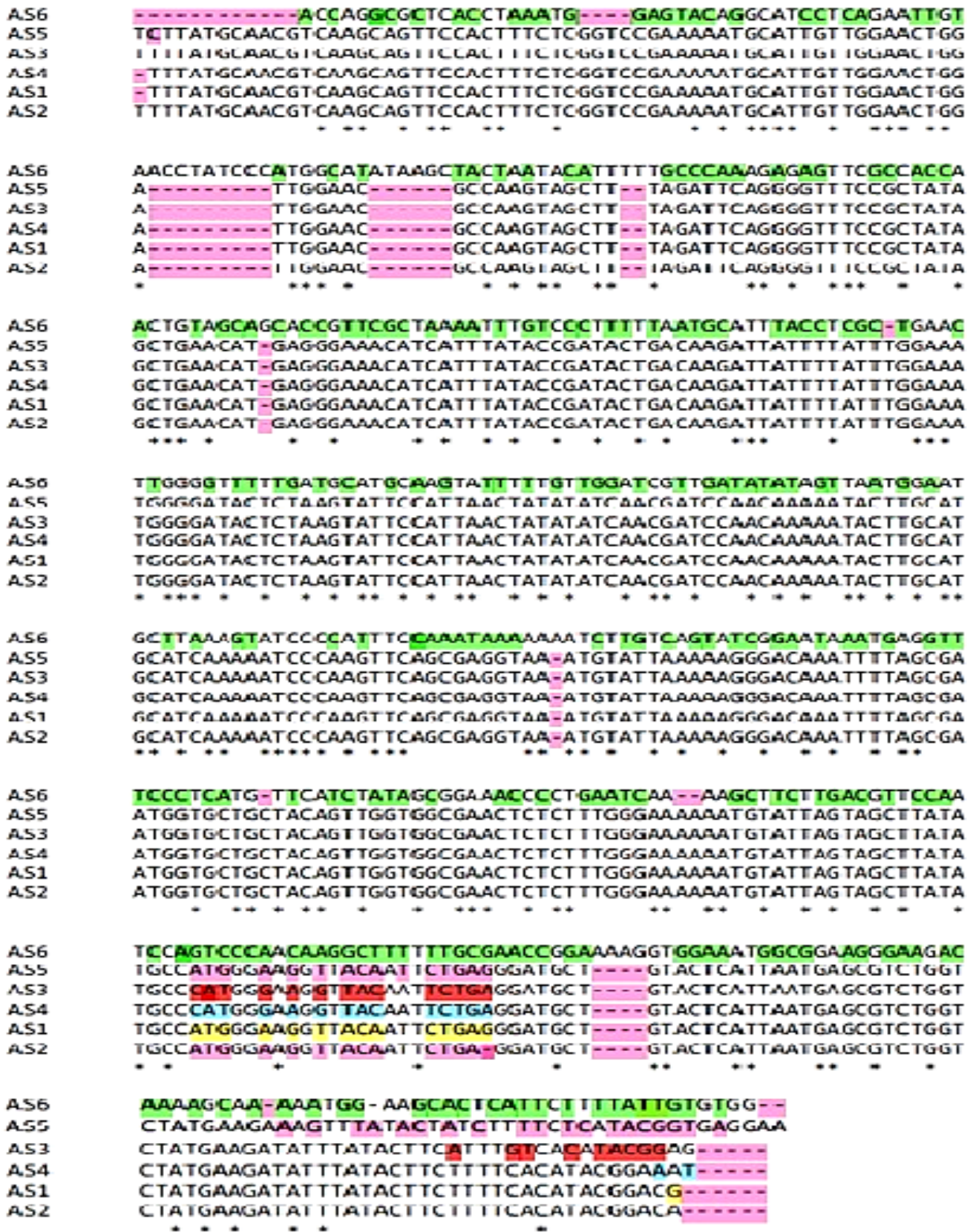
Fig. 4. The alignment of 6 sequences of rpoB of C. ternatea , including In/Dels and SNPs from different locations.
