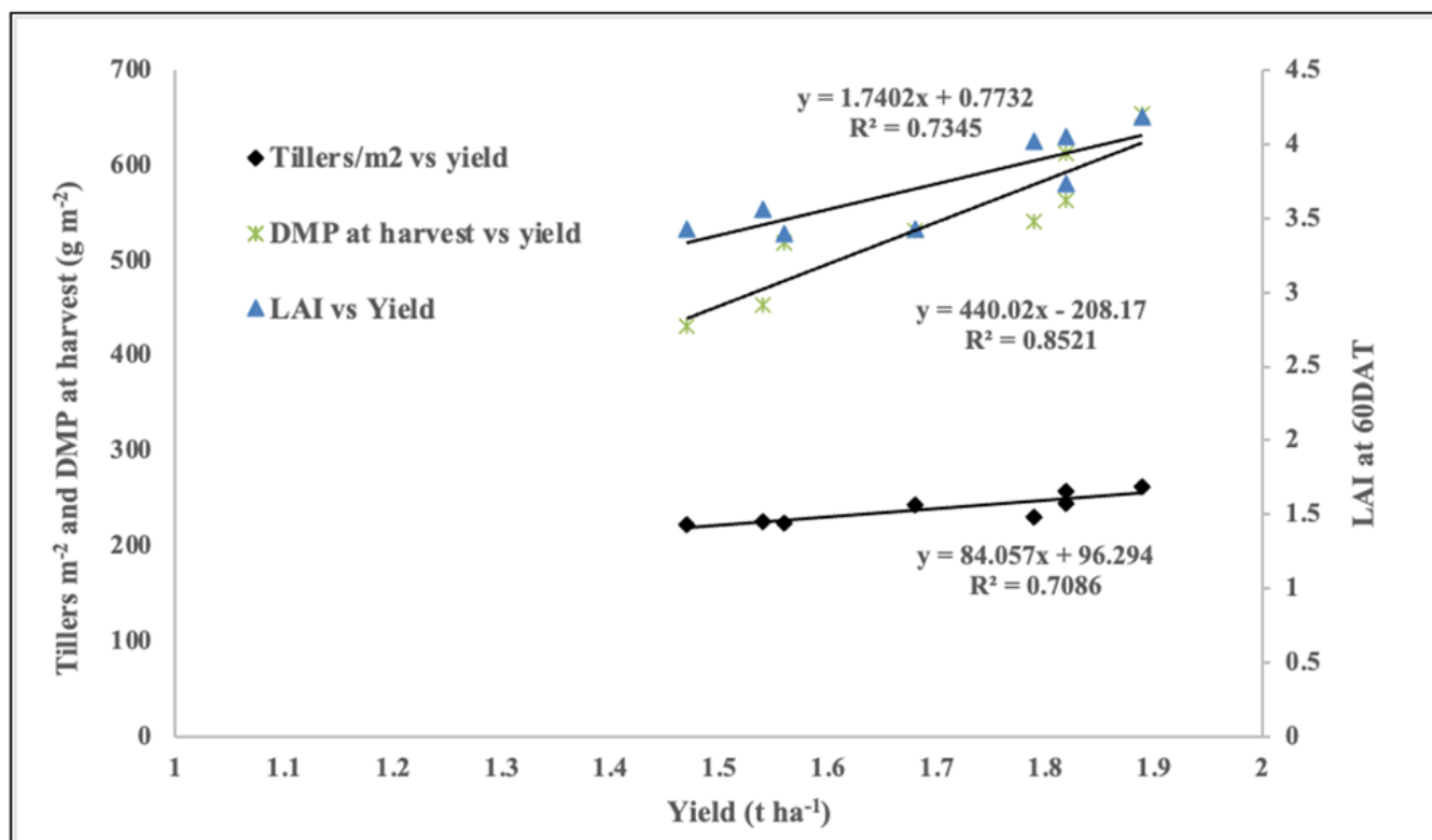
Fig. 3. Regression equations between tillers m^{-2} , dry matter production at harvest and leaf area index vs yield of organic finger millet.
