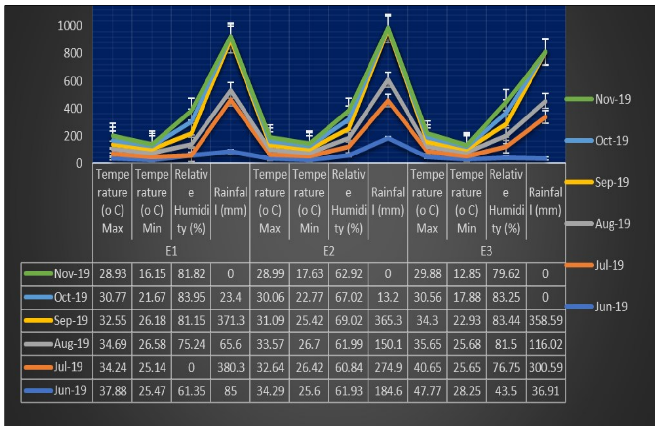
Fig. 3. Average monthly weather report during crop growing in Kharif, 2019. The environments, E1: Bihar Agricultural college, BAU, Sabour, Bhagalpur, Bihar (Zone-IIIa), E2: Bholu Paswan Shastri Agricultural College, Purnea, Bihar (Zone-II) and E3: Pulse Research Centre, Mokama, Patna (Zone-IIIb) of Bihar where experiments were conducted. Max: Maximum, Min: Minimum and mm: millimetres.
