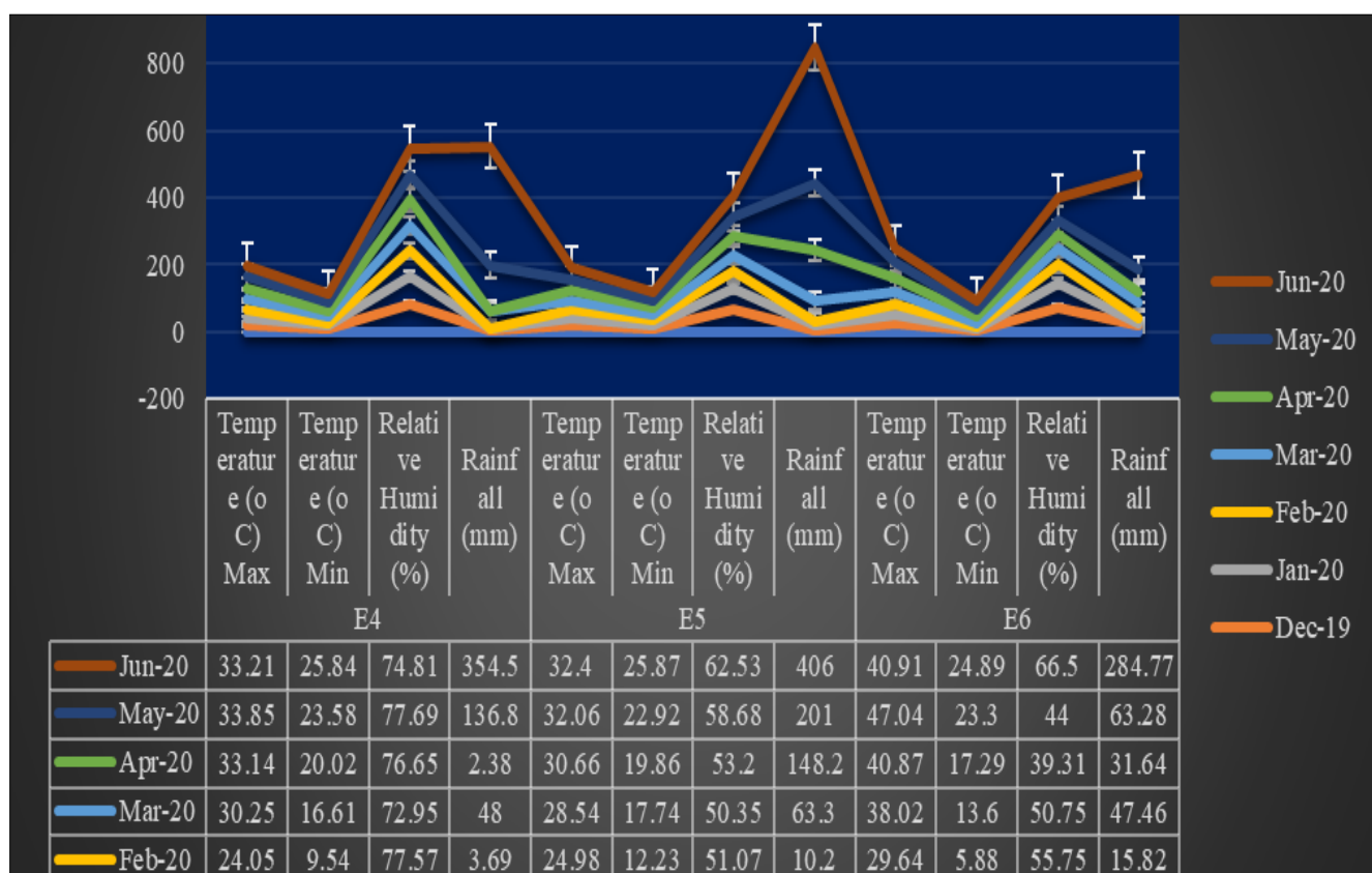
Fig. 4. Average monthly weather report during crop growing in Rabi, 2019-20. The environments, E4: Bihar Agricultural college, BAU, Sabour, Bhagalpur, Bihar (Zone-IIIa), E5: Bholu Paswan Shastri Agricultural College, Purnea, Bihar (Zone-II) and E6: Pulse Research Centre, Mokama, Patna (Zone-IIIb) was the location of Bihar where experiments were conducted. Max: Maximum, Min: Minimum and mm: millimeters.
