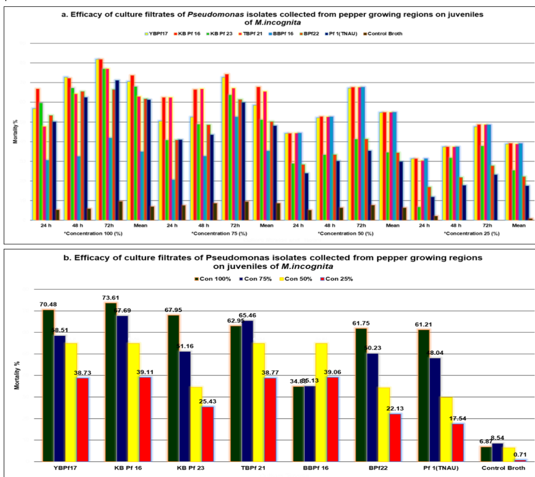
Fig. 2. Efficacy of culture isolates of Pseudomonas isolates from pepper growing regions against M. incognita (a) DAT (b) Mean values.
