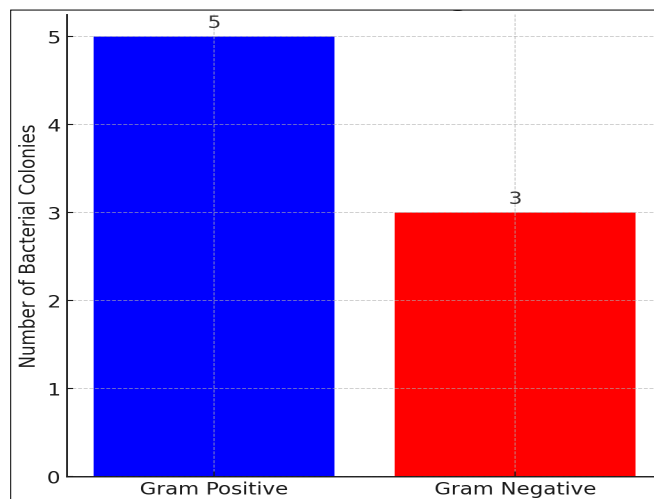
Fig. 4. Distribution pattern of Gram-positive and Gram-negative bacteria in airborne bioaerosols.
