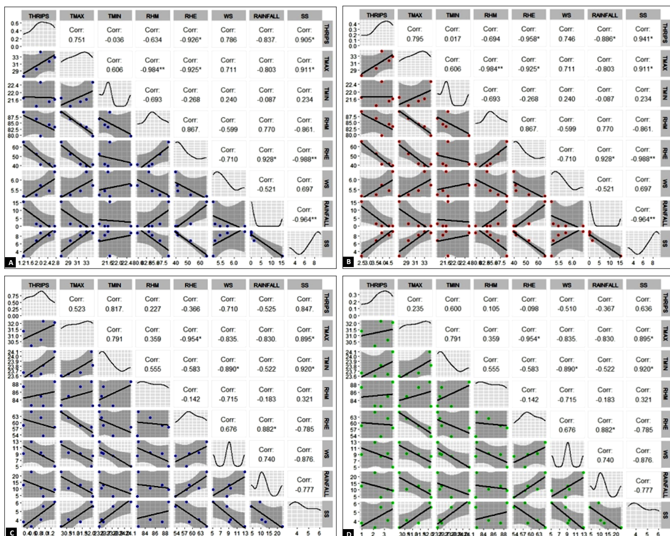
Fig. 2. Graph showing the correlation between weather parameters and Scirtothrips dorsalis during different seasons. A) IC-344364 ( rabi ); B) IC-537583 ( rabi ); C) IC-344364 ( kharif ); D) IC-537583 ( kharif ).
