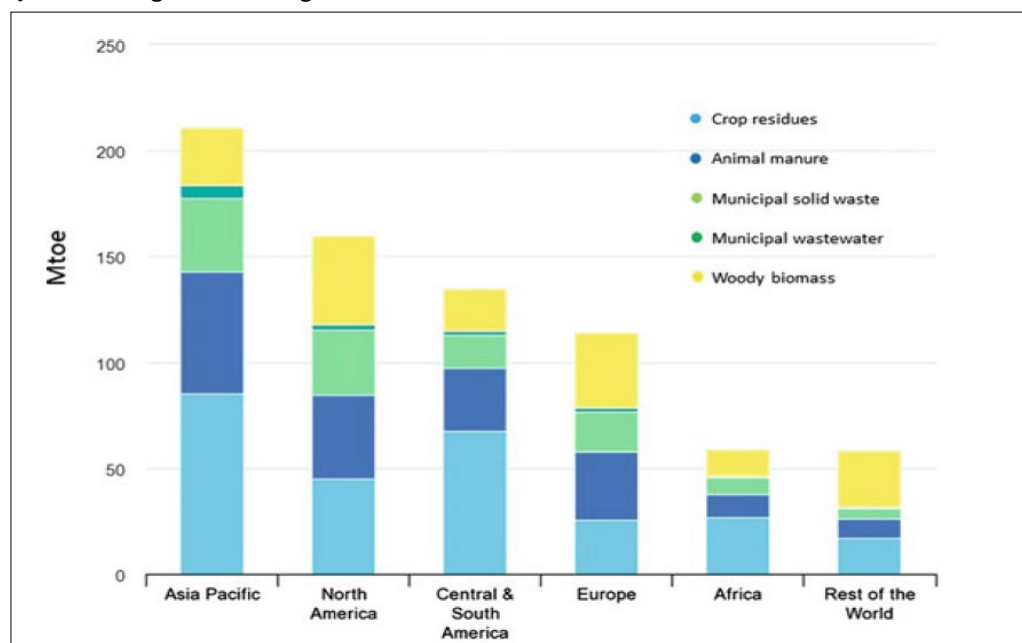
Fig. 2. Energy potential of biogas or biomethane by feedstock (15).
