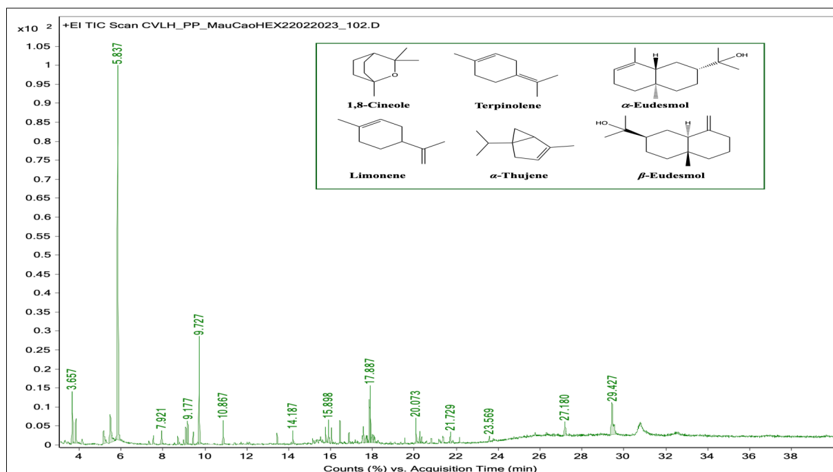
Fig. 2. GC-MS chromatogram and the identified main counts in LCV
