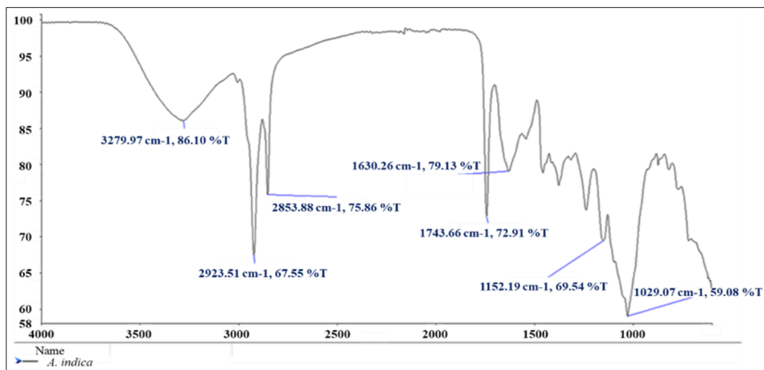
Fig. 4. FTIR of A. indica extract obtained using simultaneously ultrasound and microwaves.
