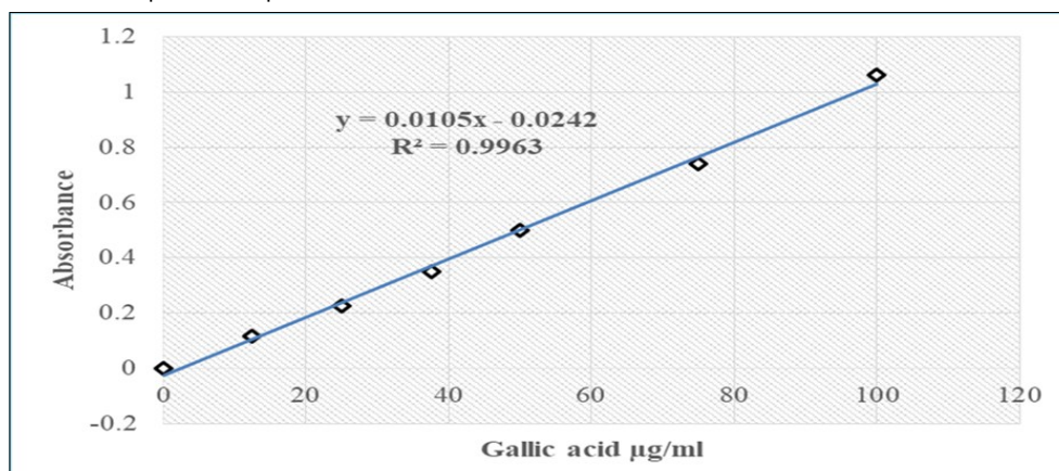
Fig. 8. Calibration curve of polyphenol contents established with gallic acid ( \mu\text{g/ml} ). absorbance measurements were performed using a UV/Vis spectrophotometer at 765 nm.
