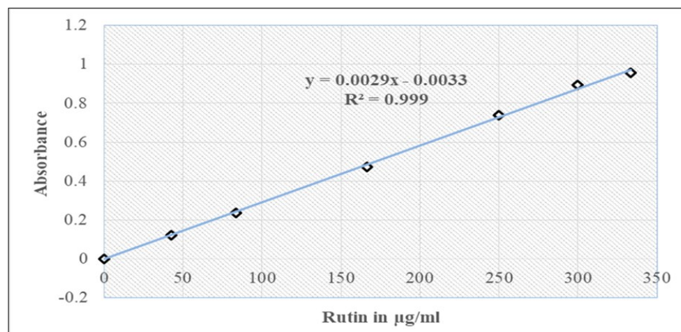
Fig. 9. Calibration curve of flavonoid contents established with Rutin ( \mu\text{g/ml} ). Absorbance was measured at 510 nm.
