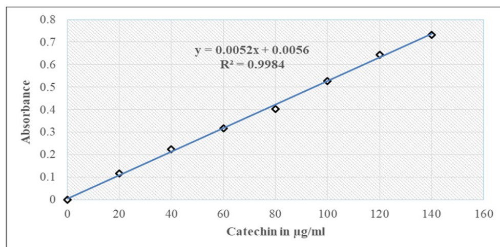
Fig. 10. Calibration curve of flavonoid contents established with Catechin ( \mu\text{g/ml} ). Absorbance was measured at 510 nm.
