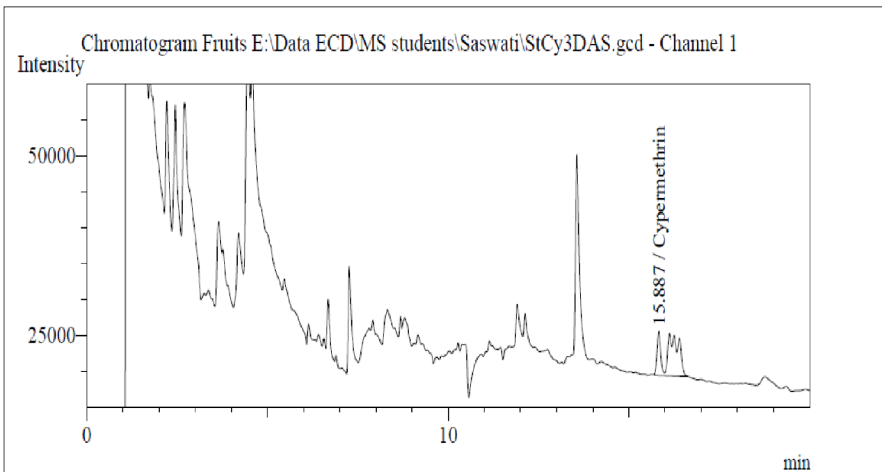
Fig. 5. Chromatogram of cypermethrin obtained from strawberry extract at 3 DAS.
