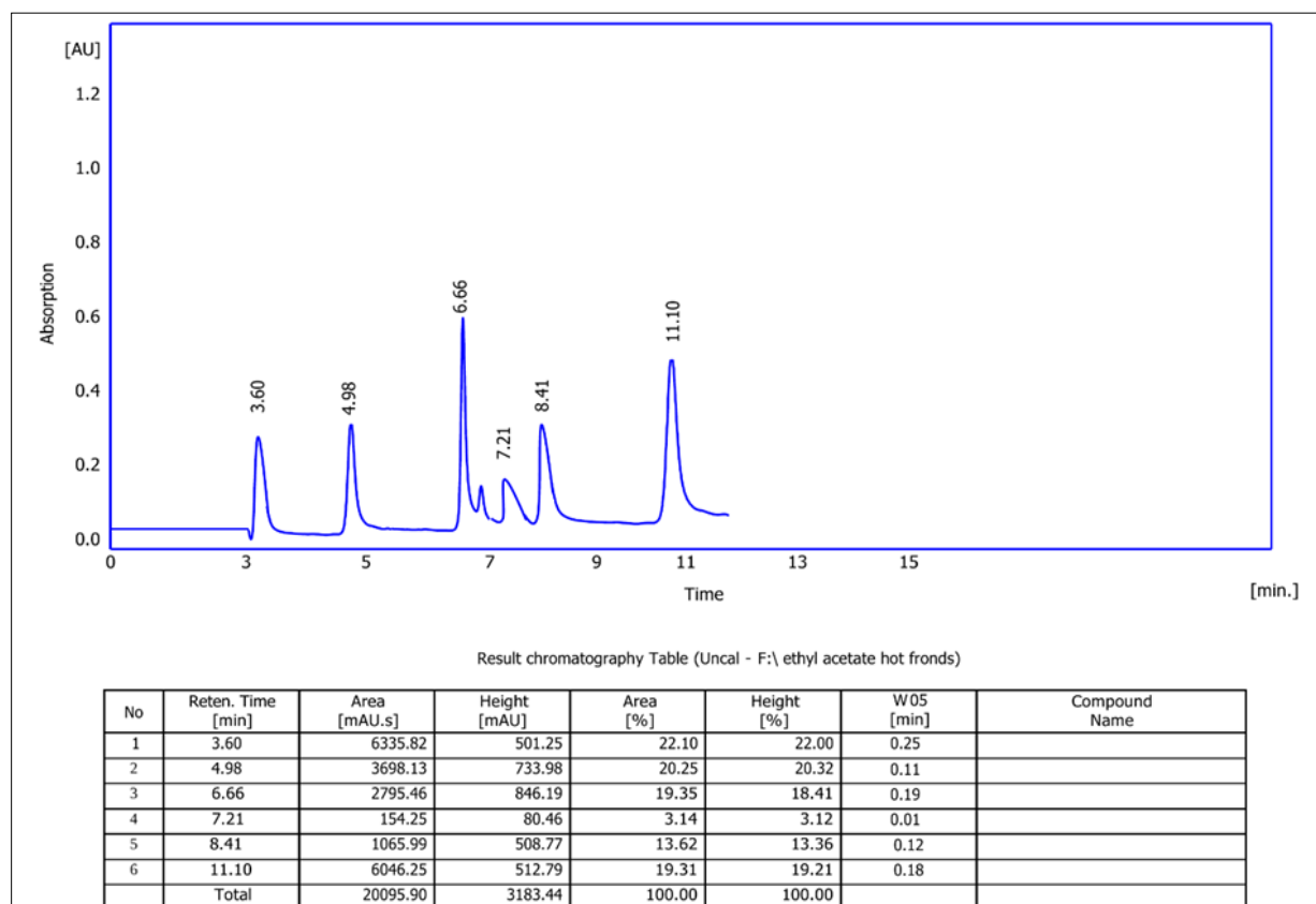
Fig. 6. HPLC for sample ethyl acetate leaves extract.
