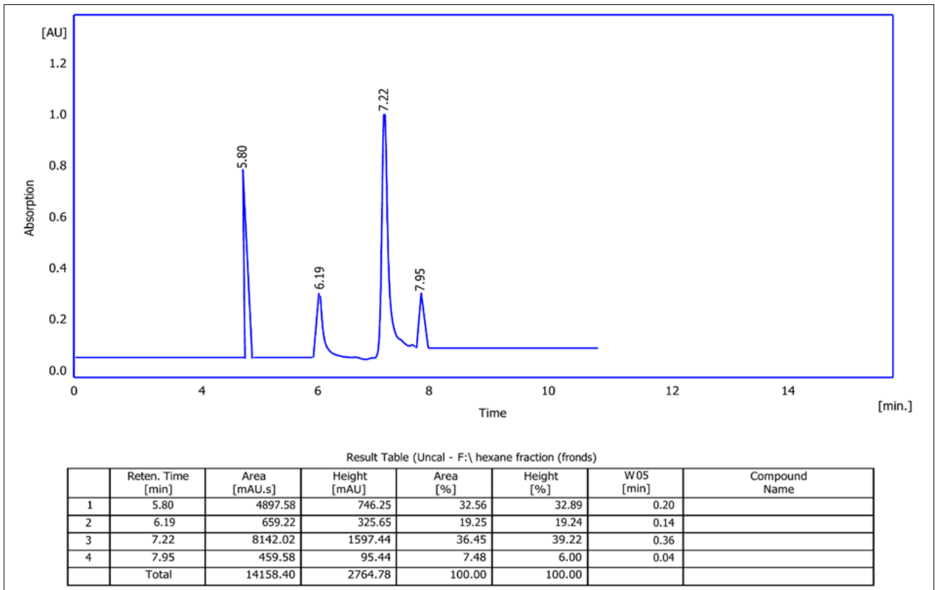
Fig. 3. HPLC of Cycas revoluta n-hexane leaves extract.
