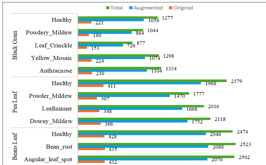
Fig. 2. Legume crop leaf original and augmented images from different classes.
