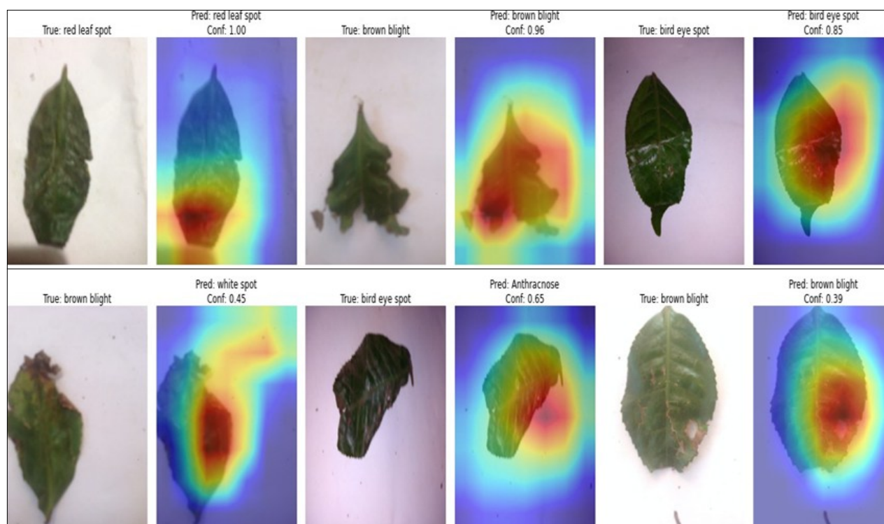
Fig. 7. Grad-CAM visualizations highlighting key regions influencing classification decisions. Red areas indicate high importance, while blue areas are less influential.
