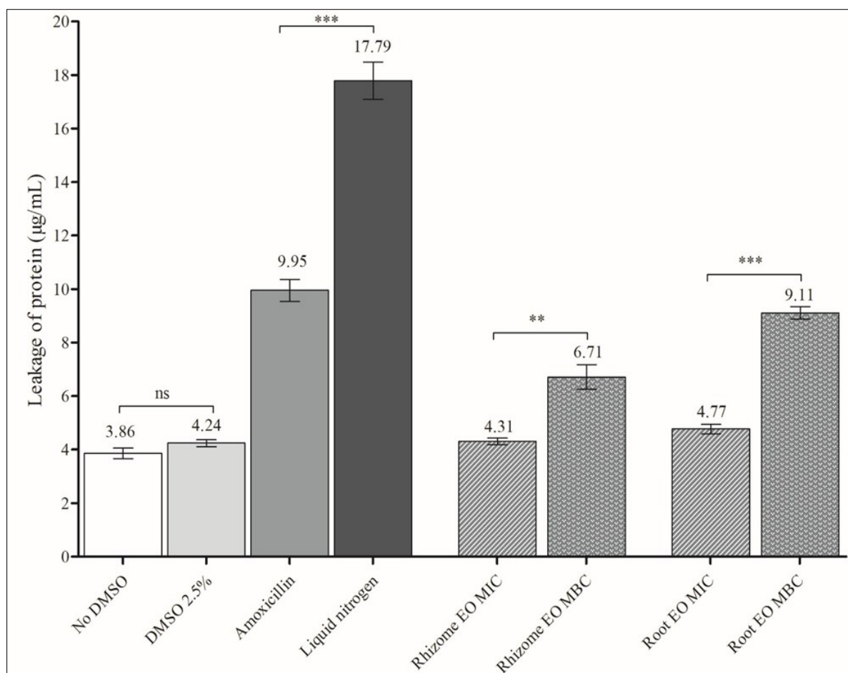
Fig. 4. Protein leakage from H. pylori after 4 h of treatment with the B. rotunda rhizome and tuberous root EOs at both MIC and MBC levels 'ns' depicts no significant difference at P > 0.05 ; **indicates significantly different at P < 0.01 and ***indicates significantly different at P < 0.001 (Bonferroni test).
