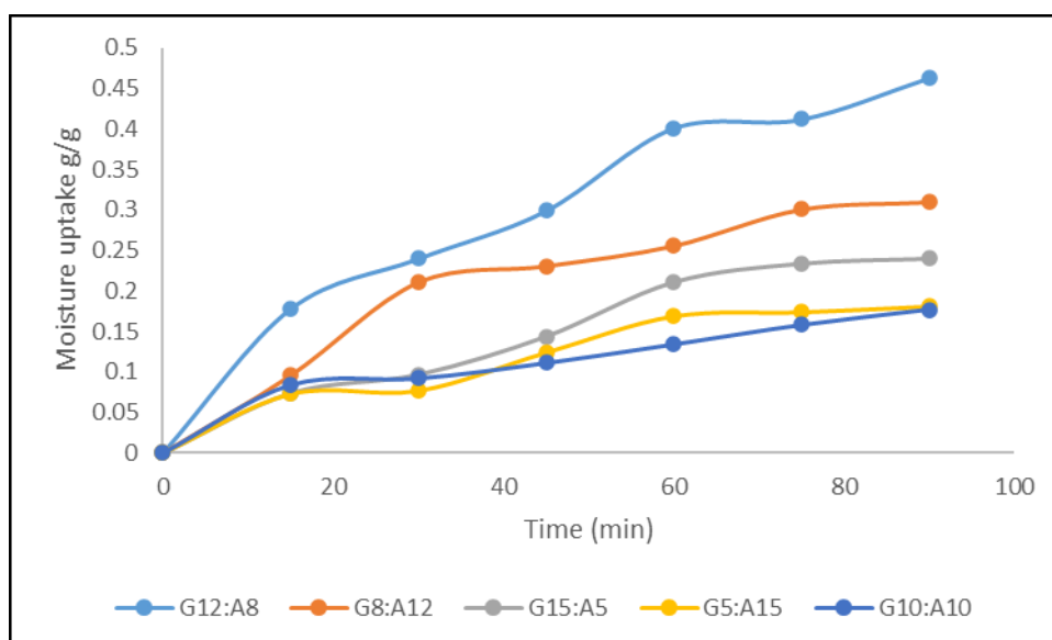
Fig. 9. Graph showing moisture uptake.
