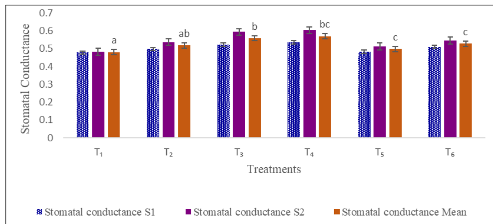
Fig. 3. Effect of Natio on stomatal conductance ( \text{mmol H}_2\text{O m}^{-2} \text{s}^{-1} ) of tomato.
