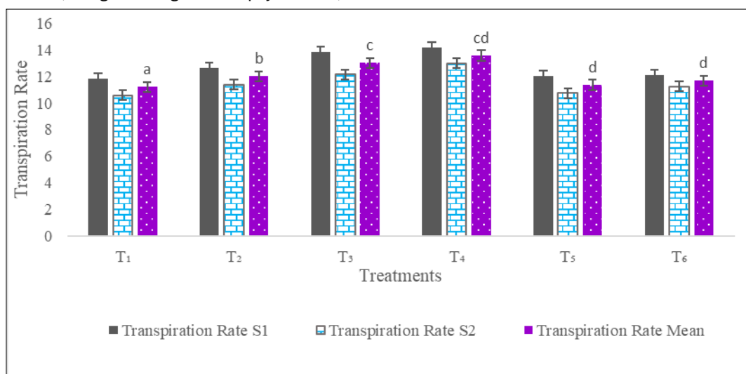
Fig. 4. Effect of Natio on transpiration rate ( \text{mol H}_2\text{O m}^{-2} \text{s}^{-1} ) of tomato.
