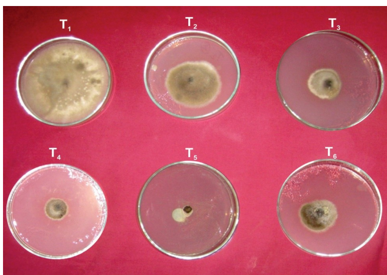
Fig. 1. Effect of different concentrations of Nativio on mycelial growth of A. solani . T1 – Control; T2 – Nativio 75 WG at 25 ppm; T3 – Nativio 75 WG at 50 ppm; T4 – Nativio 75 WG at 75 ppm; T5 – Nativio 75 WG at 100 ppm and T6 – Mancozeb at 100 ppm.
