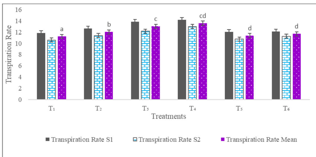
Fig. 4. Effect of Nativo on transpiration rate ( \text{mol H}_2\text{O m}^{-2} \text{s}^{-1} ) of tomato.
