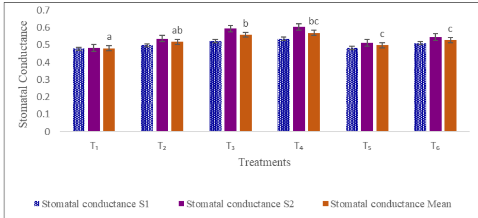
Fig. 3. Effect of Nativo on stomatal conductance ( \text{mmol H}_2\text{O m}^{-2} \text{s}^{-1} ) of tomato.
