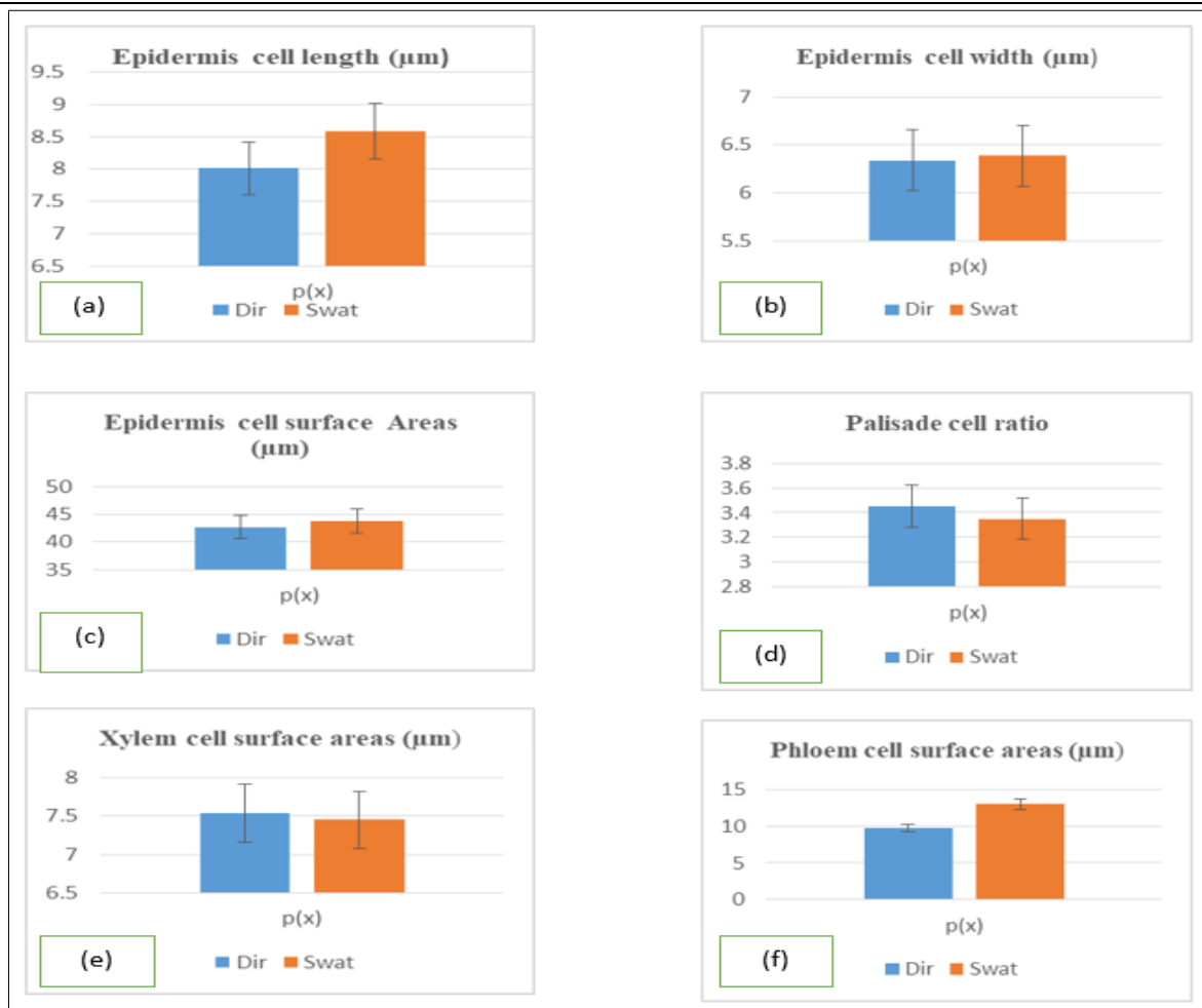
Fig. 2. Histogram of mean values of leaf anatomy traits on the Dir and Swat (a-f). (a) Shows epidermis cell length; (b) shows epidermis cell width; (c) shows epidermis cell surface area; (d) shows palisade cell ratio; (e) shows xylem cell surface area; (f) shows phloem cell surface area.
