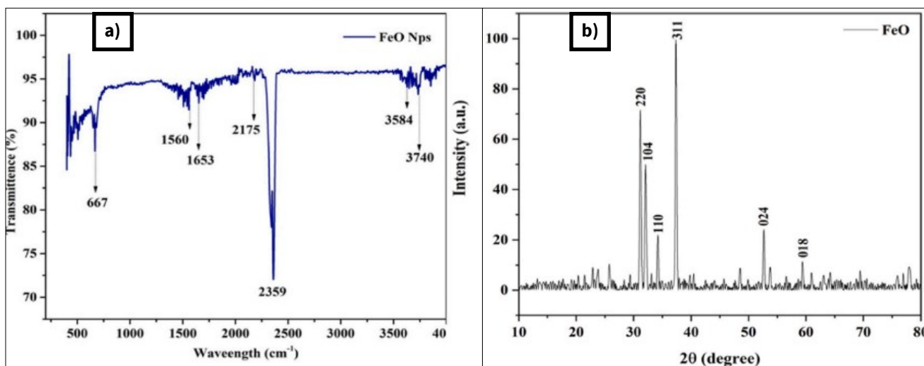
Fig. 3. The chemical composition of Fe nanoparticles. (a) Fourier transform infrared spectroscopy and (b) X-ray diffraction analysis (39).
