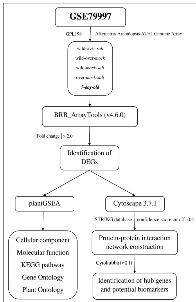
Fig. 1. Flowchart of step by step approaches to achieve the final validated genes in terms of Arabidopsis salt stress.
