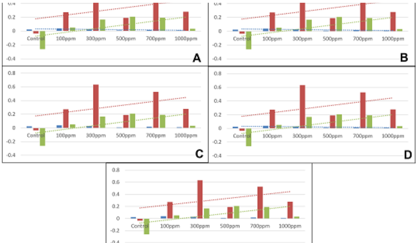
Fig. 6. Showing in vitro optimization hydrocarbon effect on growth kinetics vs. degradation (A. 222, B.221, C.223, D.122, E.117).
