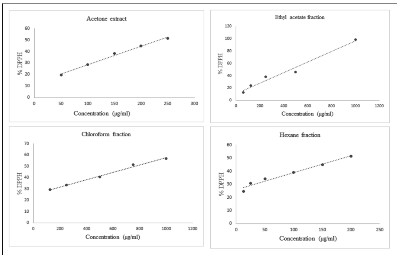
Fig. 4. Radical scavenging activity of acetone extract and its fractions of P. cornutus .
