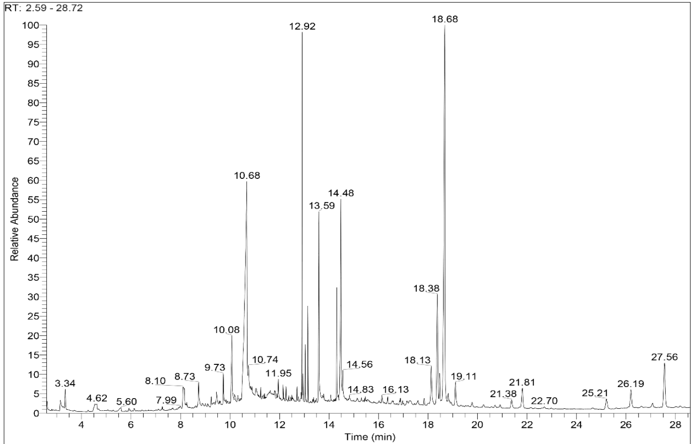
Fig. 2. Gas chromatogram of acetone extract from Phlogacanthus cornutus .
