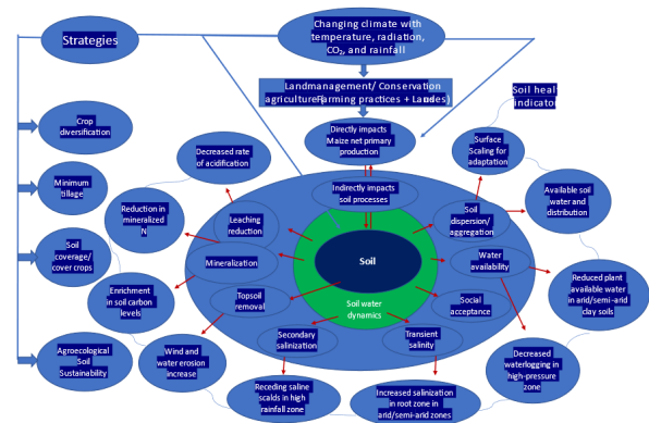
Fig. 3: Schematic representation of the linkage between climate change and soil health and strategies for soil sustainability (45, Modified from Nuttall et al. 2008).
