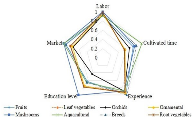
Fig. 4. Weighted Sociality of urban agriculture models in Cai Rang District
