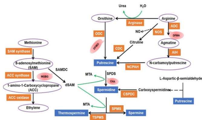
Fig 2. Biosynthesis pathway of main PAs in plants (12)
