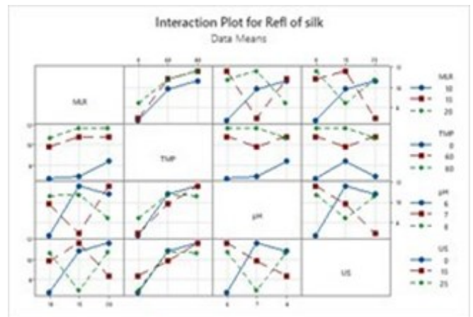
Figure 17: Interaction plot of silk
