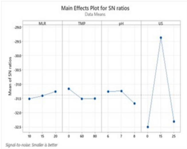
Figure 12: Main effects plot for SN ratios for cotton fabric
