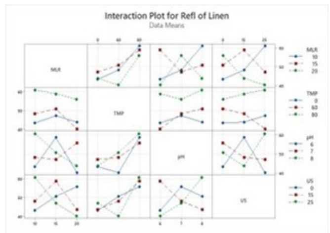
Figure 16: Interaction plot of linen
