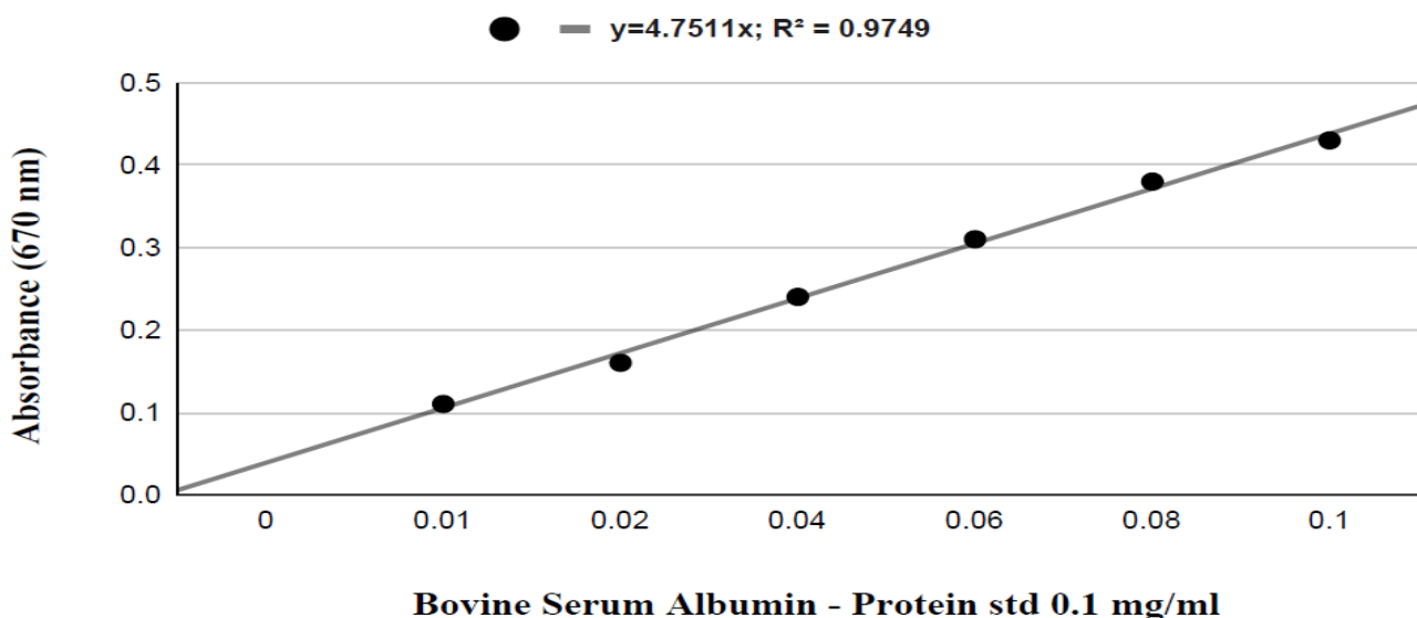
Fig. 1. Standard protein graph by Lowry's method.
