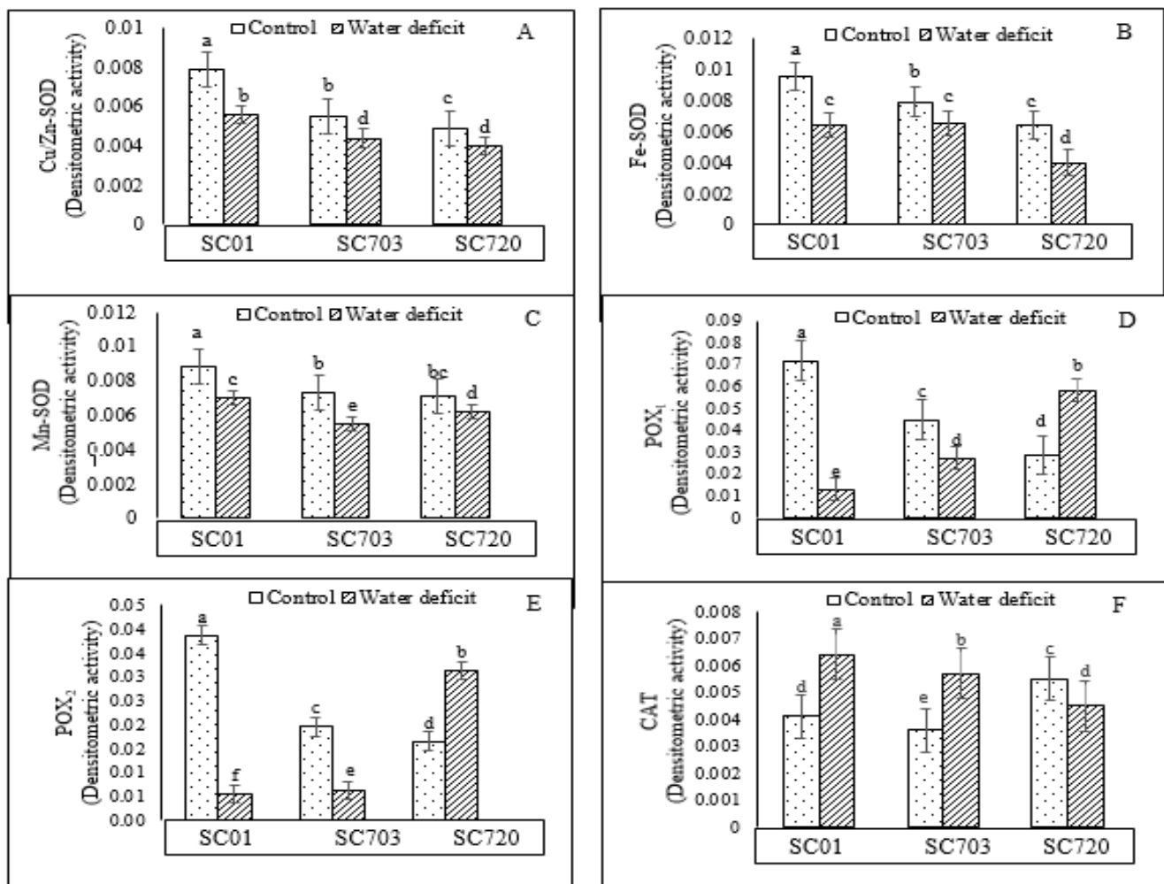
Fig. 4. Means of A-Cu/Zn-SOD, B-Fe-SOD, C-Mn-SOD, D-POX 1 , E-POX 2 , and F-CAT densitometric activities ( \pm SE) in the three maize hybrids under control and water deficit conditions.
