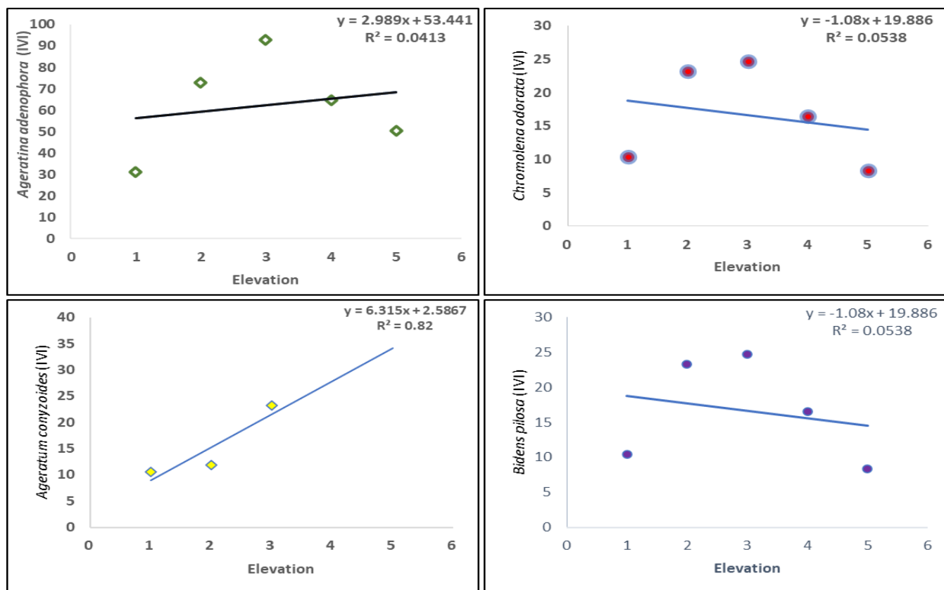
Fig. 4. Correlation analysis between importance value index (IVI) of top four invasive alien plant species at five elevational gradients in the study area 800–1200 m, 1200–1600 m, 1600–2000 m, 2000–2400 m and 2400–2800 m.
