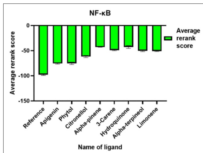
Fig. 11. Graphical representation of re-rank scores of ligands which signify the binding potential of these ligands against NF- \kappa B.
