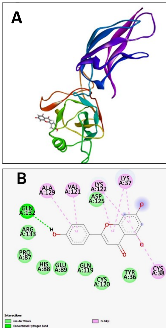
Fig. 13. Interaction of apigenin with the active site of NF- \kappa B. (A) 3D representation, (B) 2D representation.
