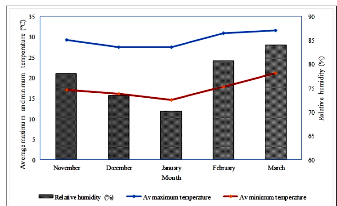
Fig. 1. Distribution of monthly temperature and relative humidity of the experimental site during the crop growth period.
