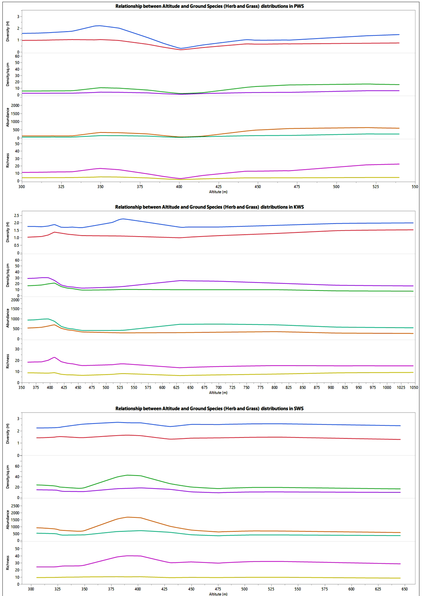
Fig. 2. Relationship between altitude and ground species (herb and grass) distributions in protected areas of the southern Aravalli regions of Rajasthan. decrease of ground species in response to altitude (45–47).
