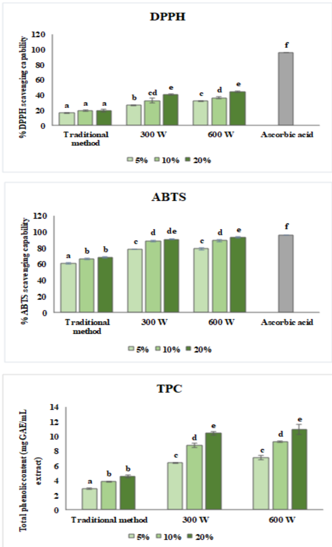
Fig. 3. Leaf extracts from Tiliacora triandra exhibiting antioxidant properties and total phenolic content: (A) DPPH scavenging capability; (B) ABTS scavenging capability; (C) Total phenolic content.
