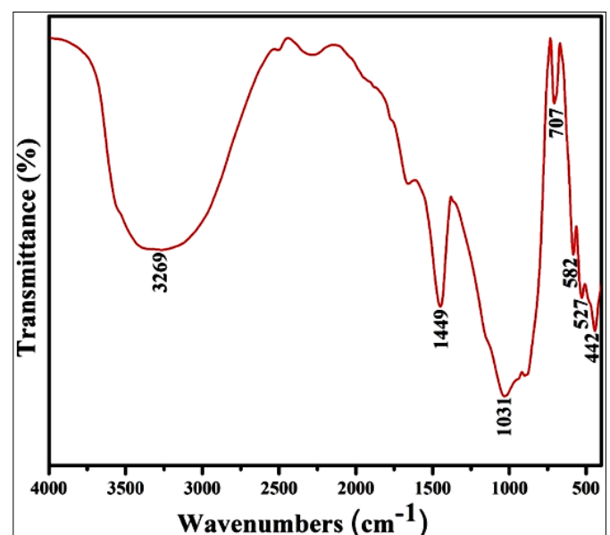
Fig. 4. FTIR graph of the catalyst ( W. coagulans ) depict major peaks corresponding to characteristic chemical groups.
