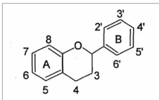
Fig. 3. Basic flavonoid structure (2-phenyl benzopyran).
