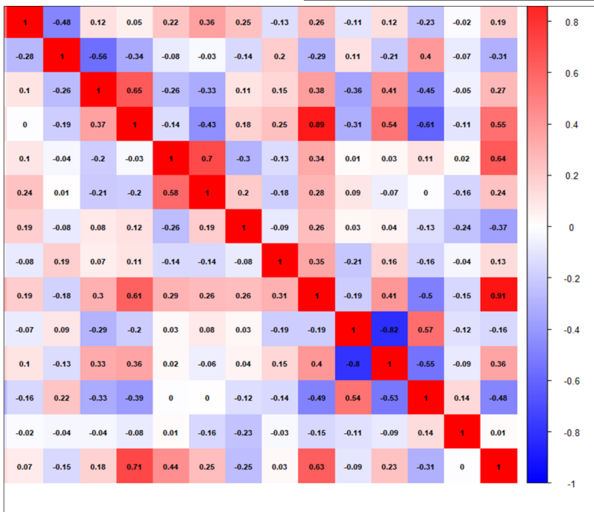
Fig. 2. Correlogram for correlation coefficients among component traits of fifty-five groundnut genotypes.
