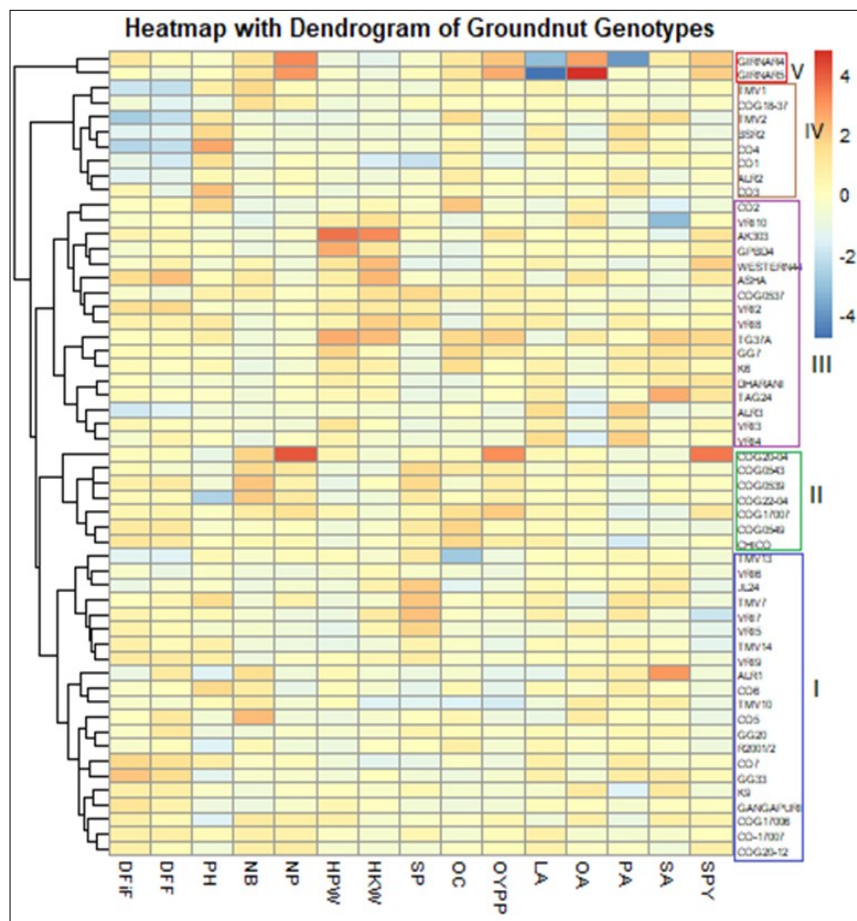
Fig. 4. The heatmap combined hierarchical clustering of 55 groundnut genotypes based on yield and oil quality parameters.
