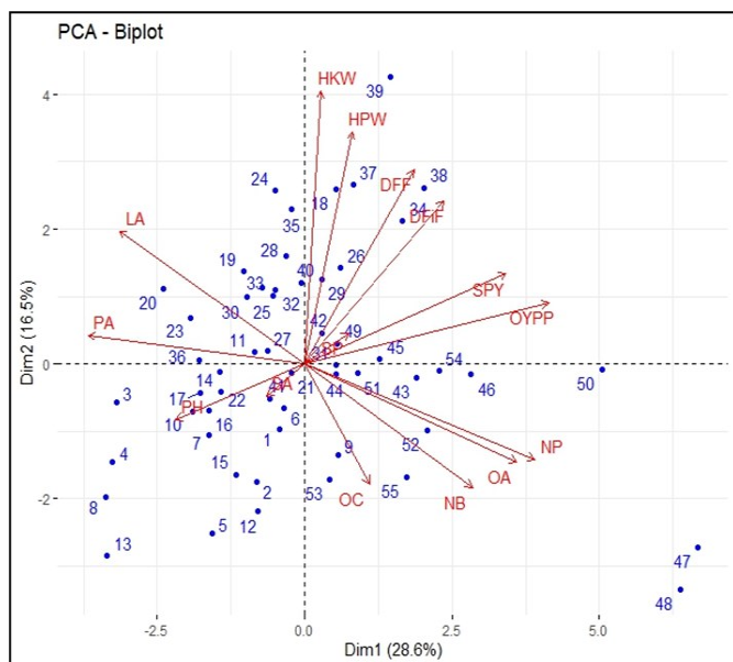
Fig. 3. Genotype by trait biplot showing distribution of genotypes across first two PCs.
