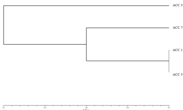
Fig. 11. Dendrogram showing phylogenetic relationships among the 4 accessions of clove based on RAPD-PCR data by OPB1 - OPB10.
