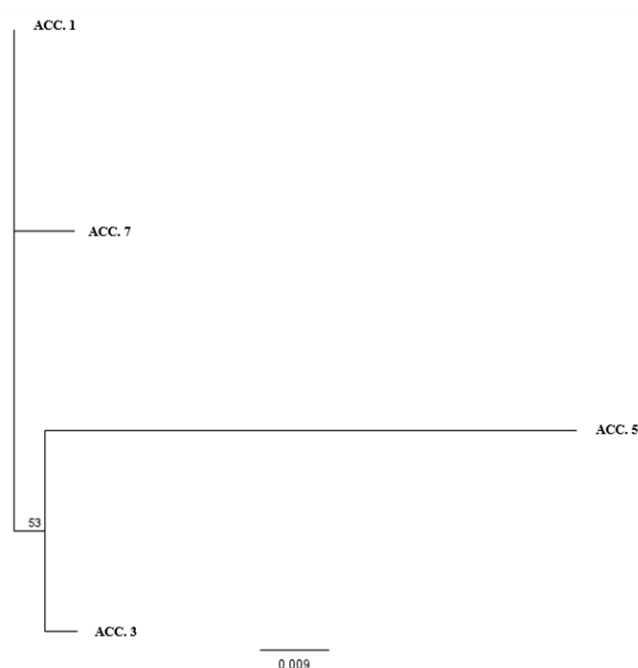
Fig. 5. Phylogenetic tree showing relatedness of clove accessions with sequences from the NCBI database.
