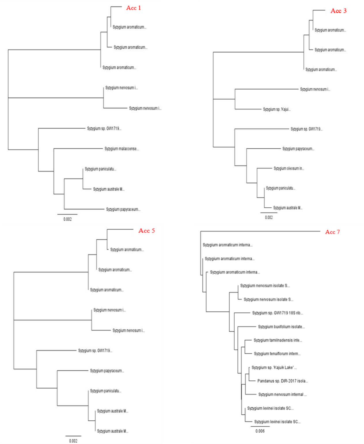
Fig. 6. Phylogenetic tree showing relatedness of 4 clove accessions.
