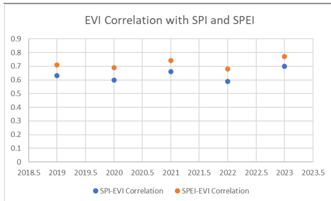
Fig. 5. EVI Correlation with SPI and SPEI
