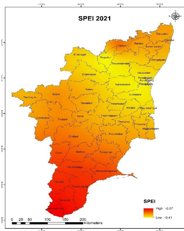
2c) SPEI map of the year 2021
