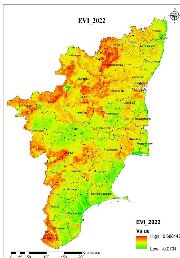
3d) EVI map of the year 2022
