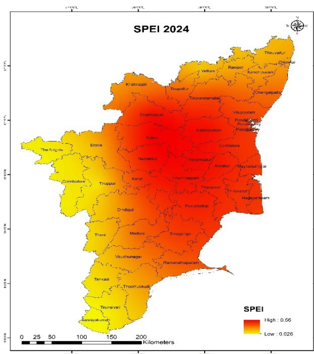
2f) SPEI map of the year 2024
