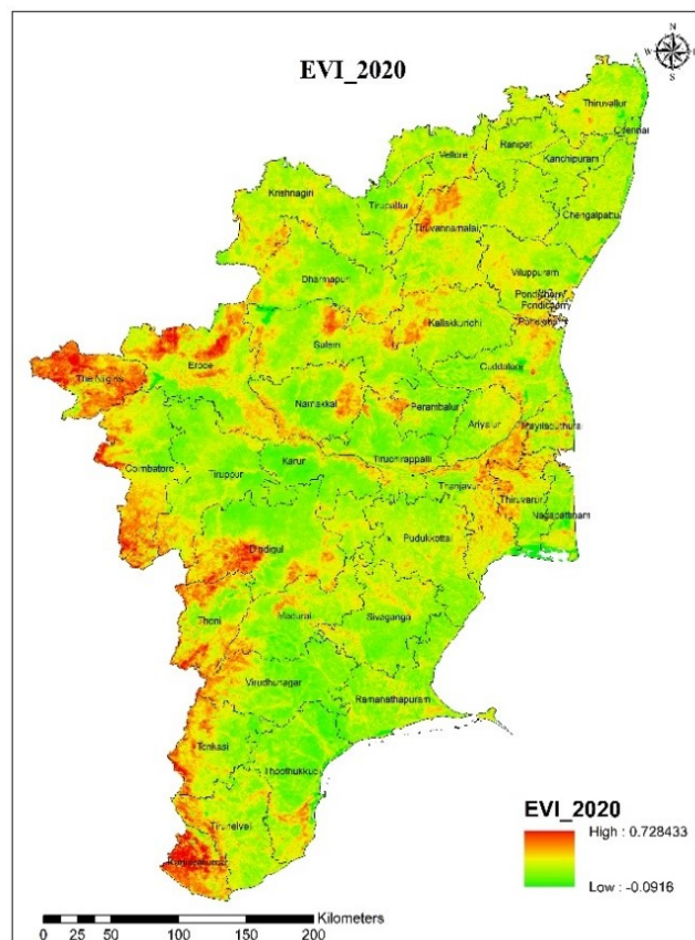
3b) EVI map of the year 2020
