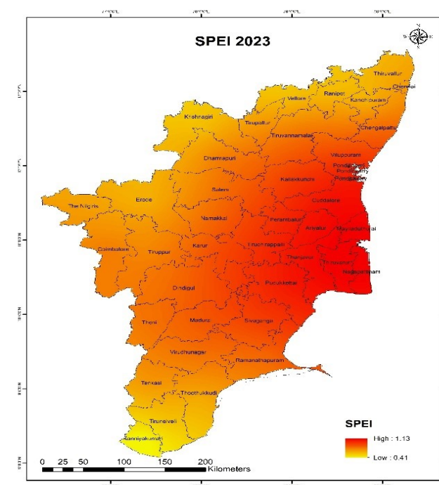
2e) SPEI map of the year 2023
