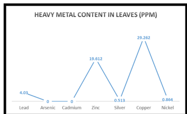
Fig. 2d. Heavy Metal Content in African Marigold Leaves – S2 (ppm)
