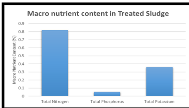
Fig. 1d. Available Macronutrients in Treated Sludge
