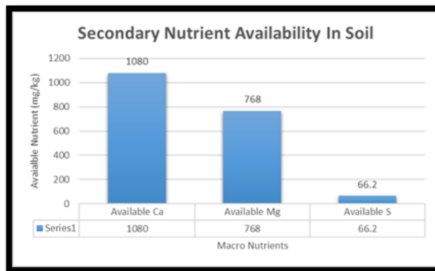
Fig. 1b. Available Secondary Nutrients in Soil
