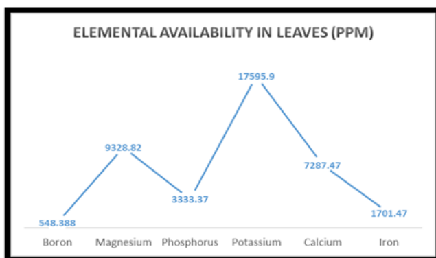
Fig. 2c. Elemental Availability in African marigold – S2 Leaves (ppm)
