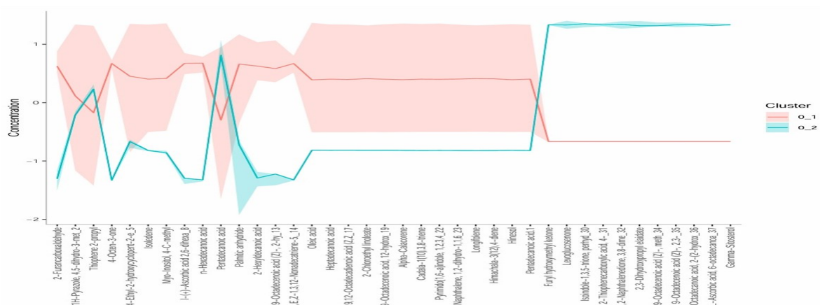
Fig. 3. SOM cluster analysis for Tamarind metabolites. The x-axes are components and y-axes are intensities. The blue lines denote median intensities of respective clusters
