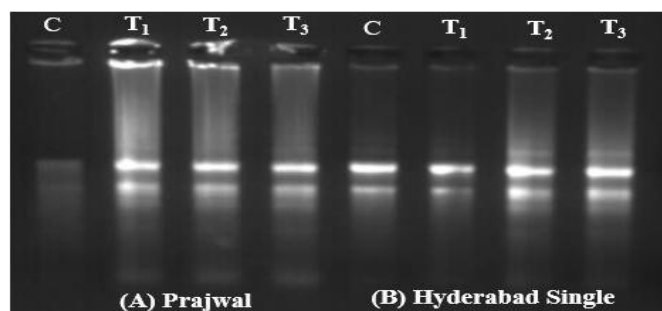
Fig. 3. Agarose gel electrophoresis of isolated total RNA on 2% agarose gel, showing two clear bands. (T 1 08 mg/L (SNP), T 2 80 mg/L (SA), T 3 10 mg/L (SNP) + 80 mg/L (SA) and control (distilled water) in both varieties Prajwal (Lane1-4) and Hyderabad Single (Lane 5-8).
