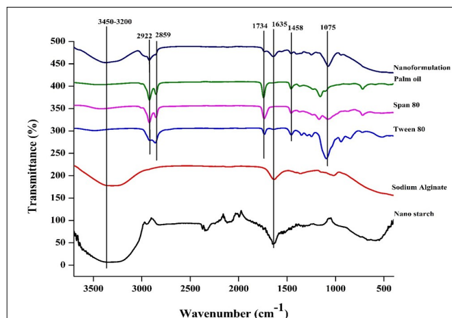
Fig. 2. FTIR spectra of the nanoformulations and all its components.
