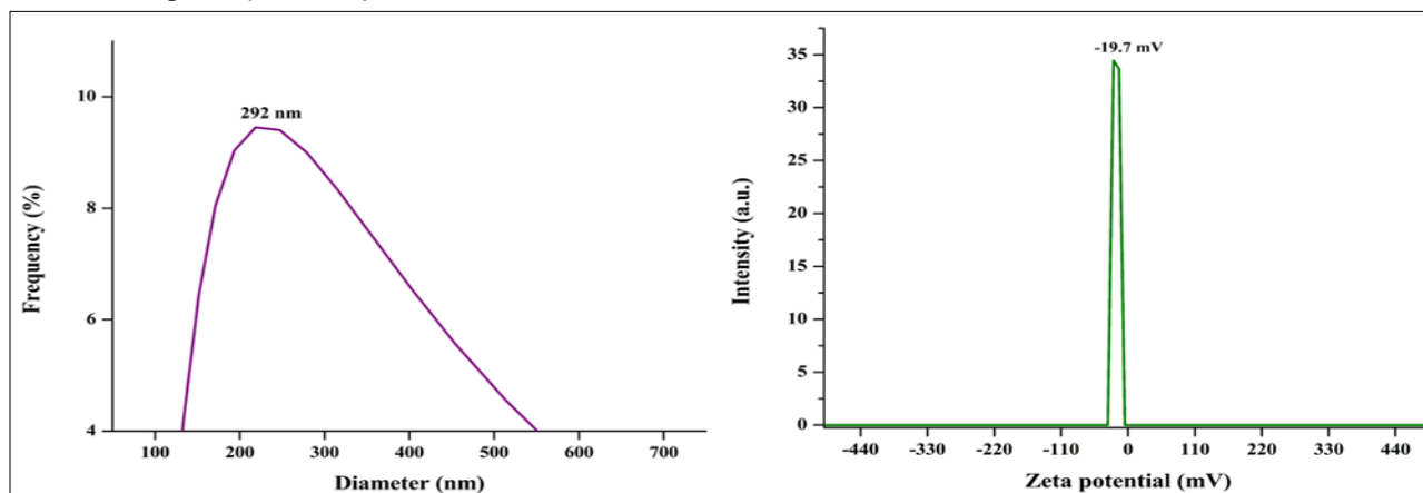
Fig. 1. Particle size determination and Zeta potential of the nanoformulations.
