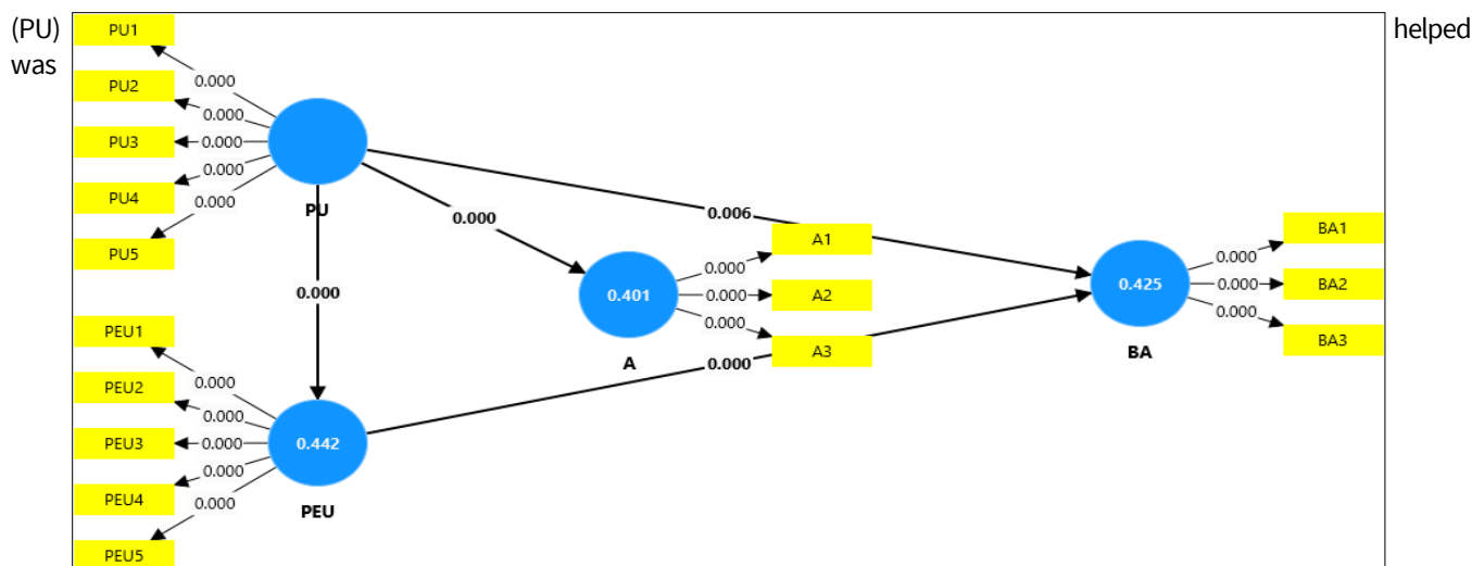
Fig. 3. Structural Model
