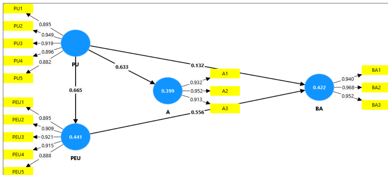
Fig. 2. Measurement Model
